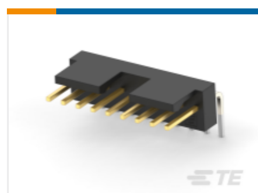
TE Part # 3-647117-9 09P MTA100 HDR HT FL 30AU LF
