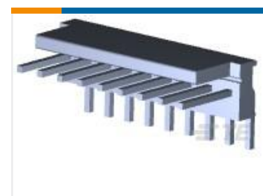
TE Part # 3-641214-9 09P MTA100 HDR ASSY PO/RA LF
